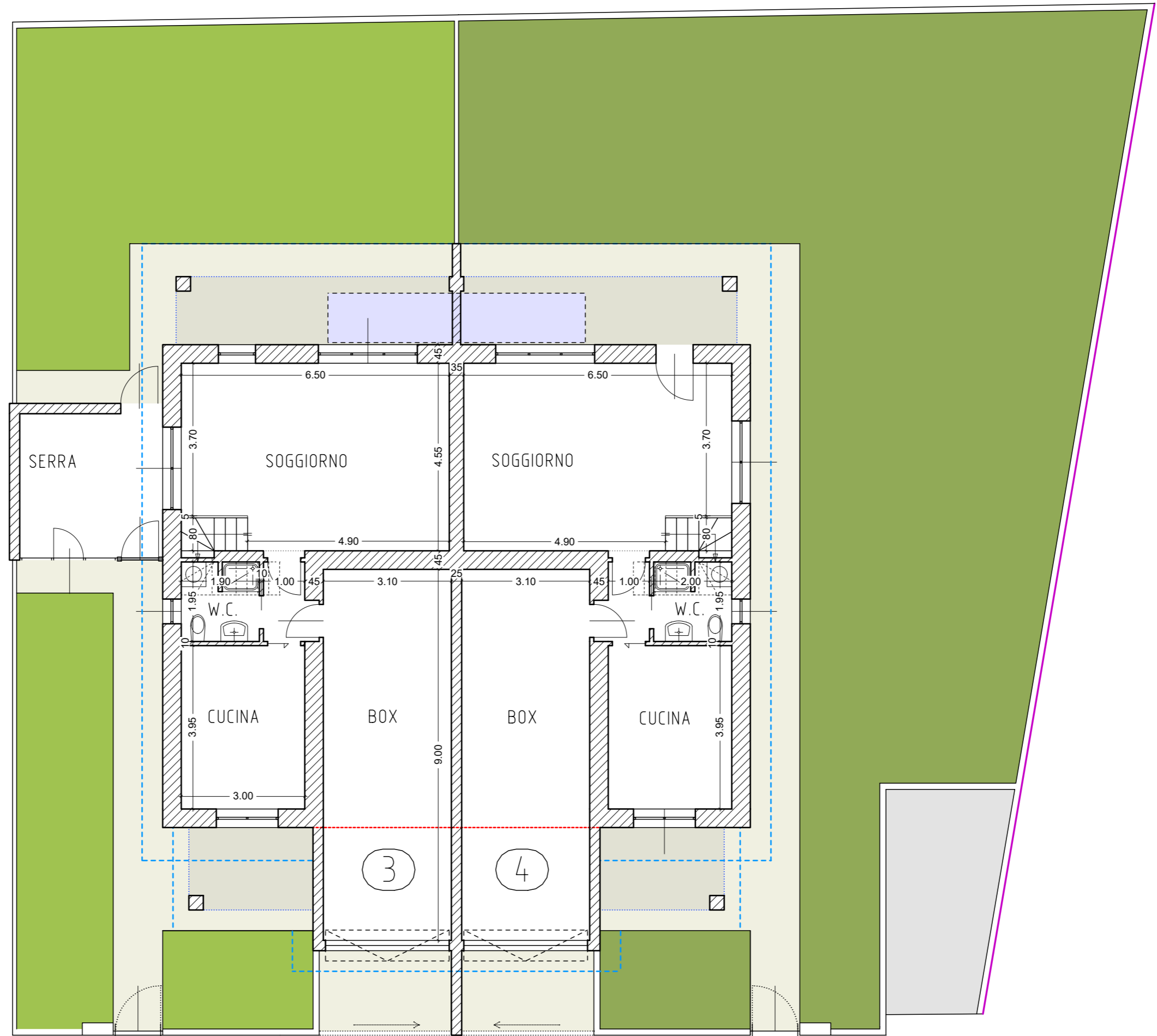
PIANO TERRA
